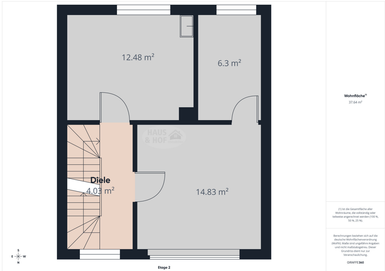
1OG Grundriss
